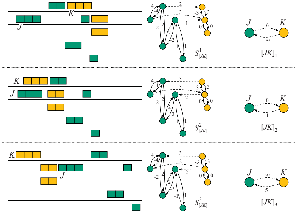
Fig. 3 Positionings of J and K (left) and corresponding selections (set of dashed arcs) in G (center) and F (right).
