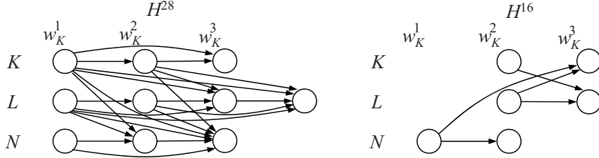
Fig. 5 Two conflict graphs.
