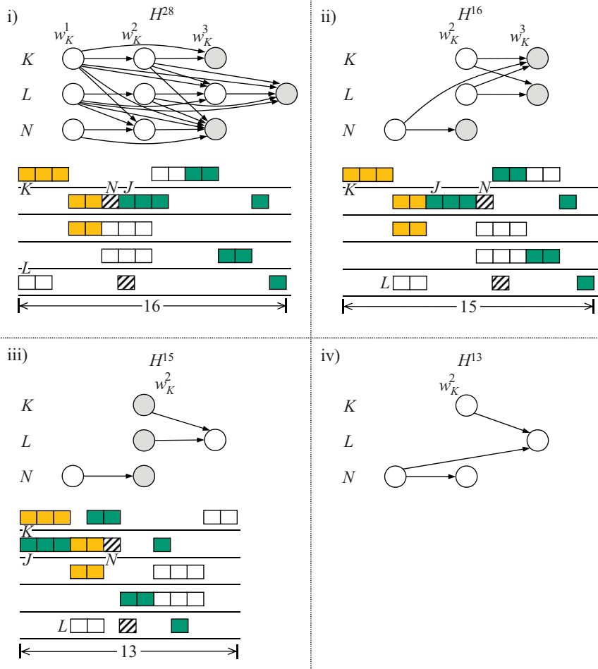
Fig. 6 A possible run of the general approach.
