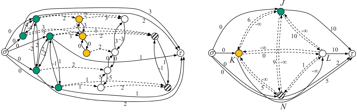
Fig. 2 Subgraph G(S) and F(S) .
