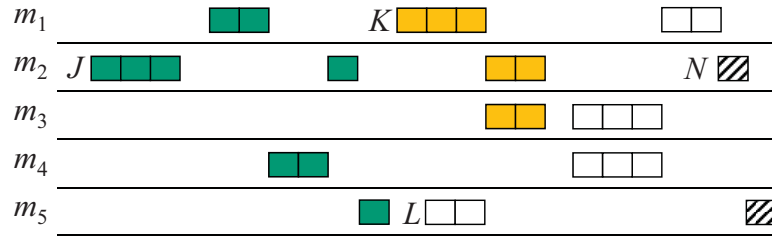
Fig. 1 Example with four jobs and five machines.
